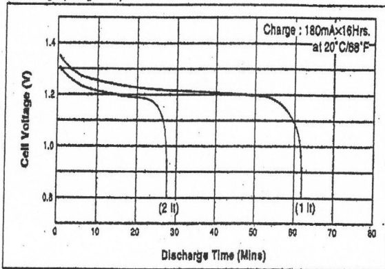
Discharge (at high rate)
