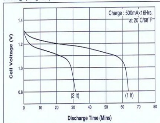
Discharge (at high rate)
